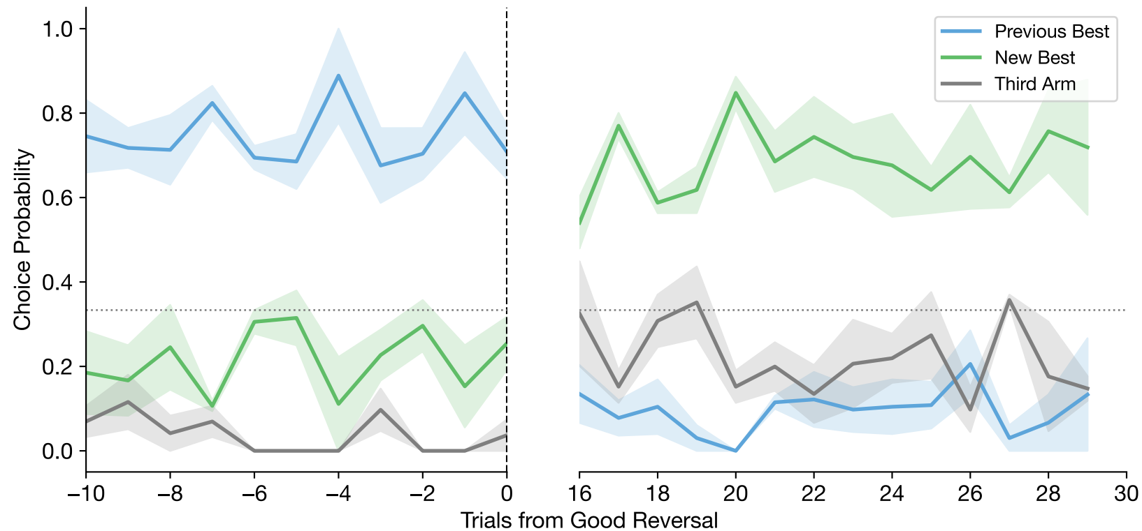
Good Reversal-Aligned Choices (mean \pm se across subjects | n=3 subjects, n=29 reversals) (Skipping first 15 trials post-reversal)
